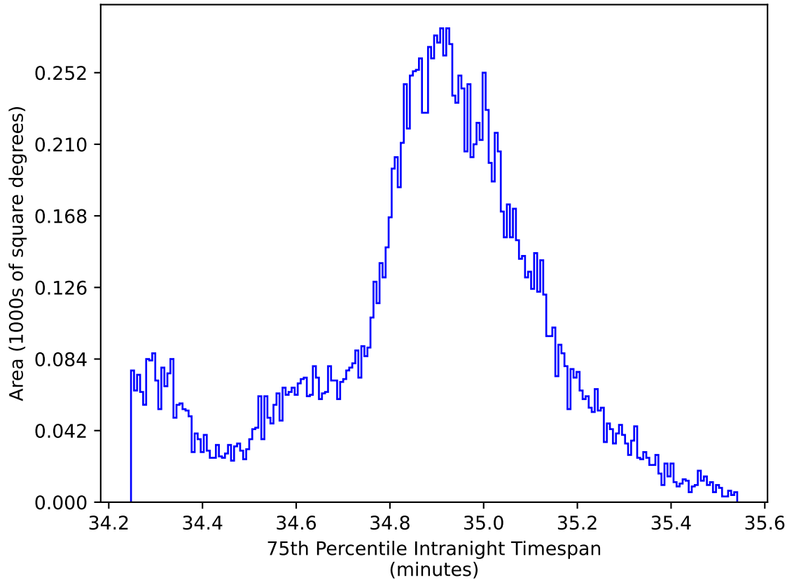
ddf_acor_sf10_lsf20_lsr50_v3.4_10yrs WFD: 75th Percentile Intranight Timespan
