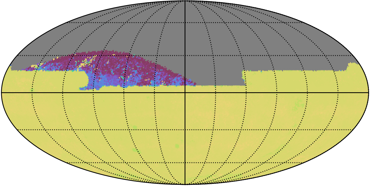
ddf_acor_sf10_lsf20_lsr50_v3.4_10yrs All sky zy bands: 75th Percentile Intranight Timespan
