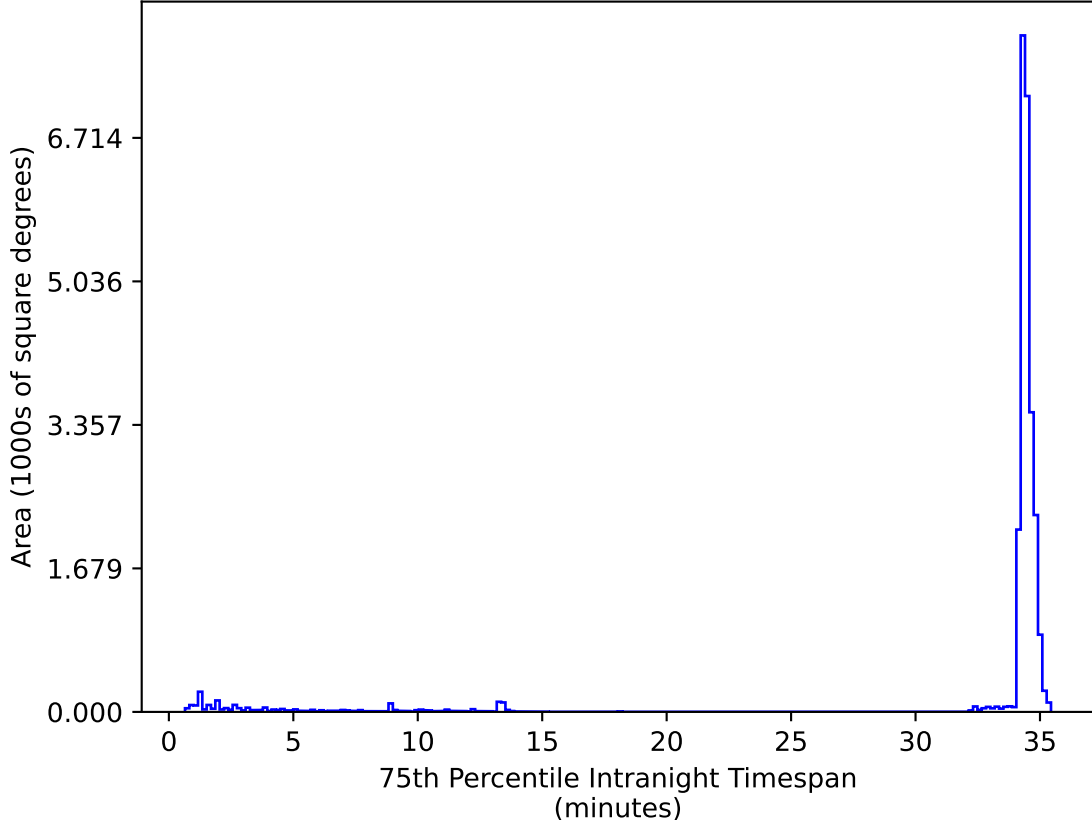
ddf_acor_sf10_ls20_lsr50_v3.4_10yrs All sky zy bands: 75th Percentile Intranight Timespan
