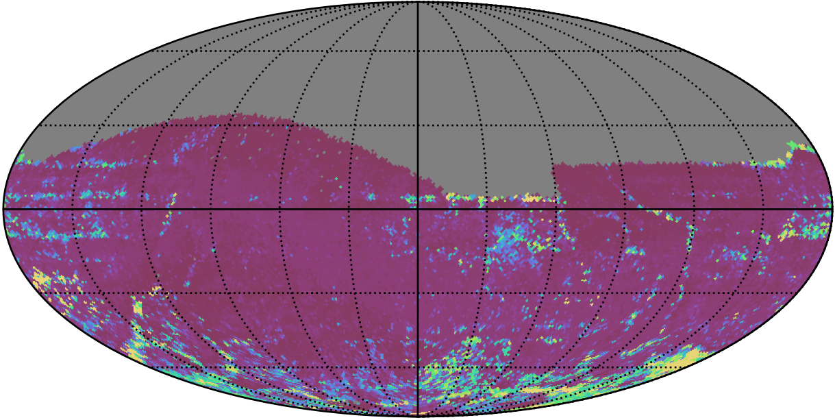
ddf_acor_sf10_lsf20_lsr50_v3.4_10yrs All sky z band: 75th Percentile Intranight Timespan
