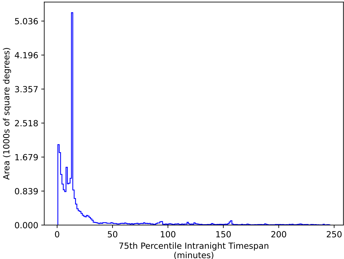
ddf_acor_sf10_lsf20_lsr50_v3.4_10yrs All sky z band: 75th Percentile Intranight Timespan
