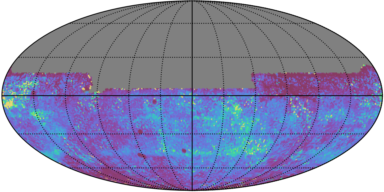
ddf_acor_sf10_lsf20_lsr50_v3.4_10yrs All sky y band: 75th Percentile Intranight Timespan
