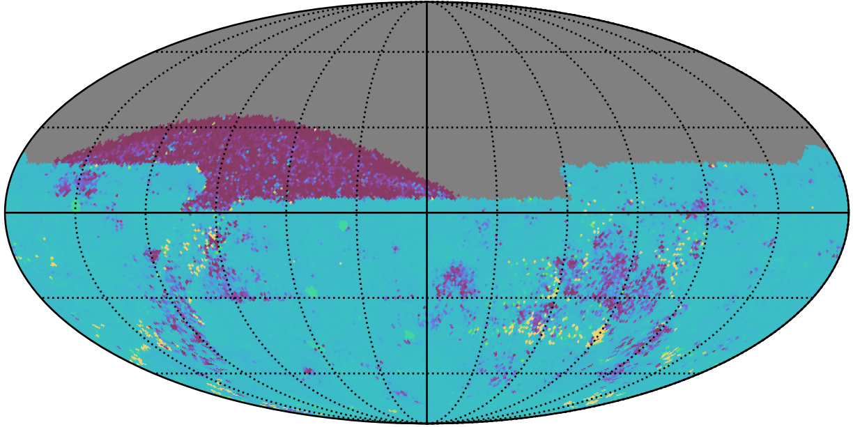
ddf_acor_sf10_lsf20_lsr50_v3.4_10yrs All sky ug bands: 75th Percentile Intranight Timespan
