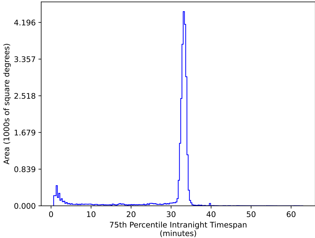
ddf_acor_sf10_lsf20_lsr50_v3.4_10yrs All sky ug bands: 75th Percentile Intranight Timespan
