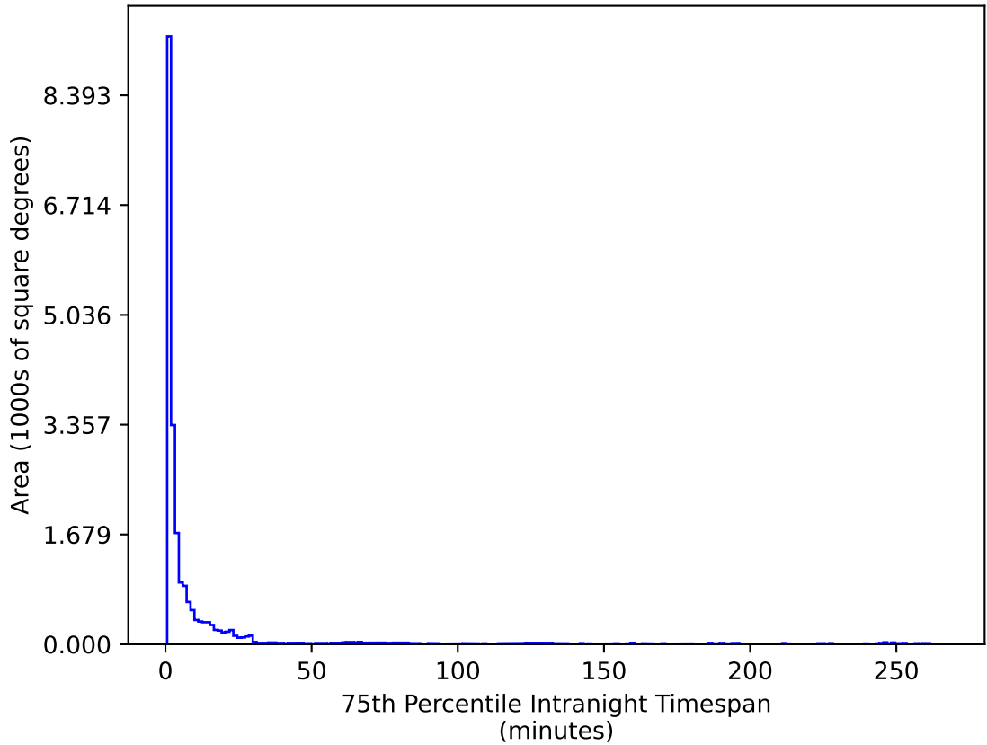
ddf_acor_sf10_lsf20_lsr50_v3.4_10yrs All sky u band: 75th Percentile Intranight Timespan
