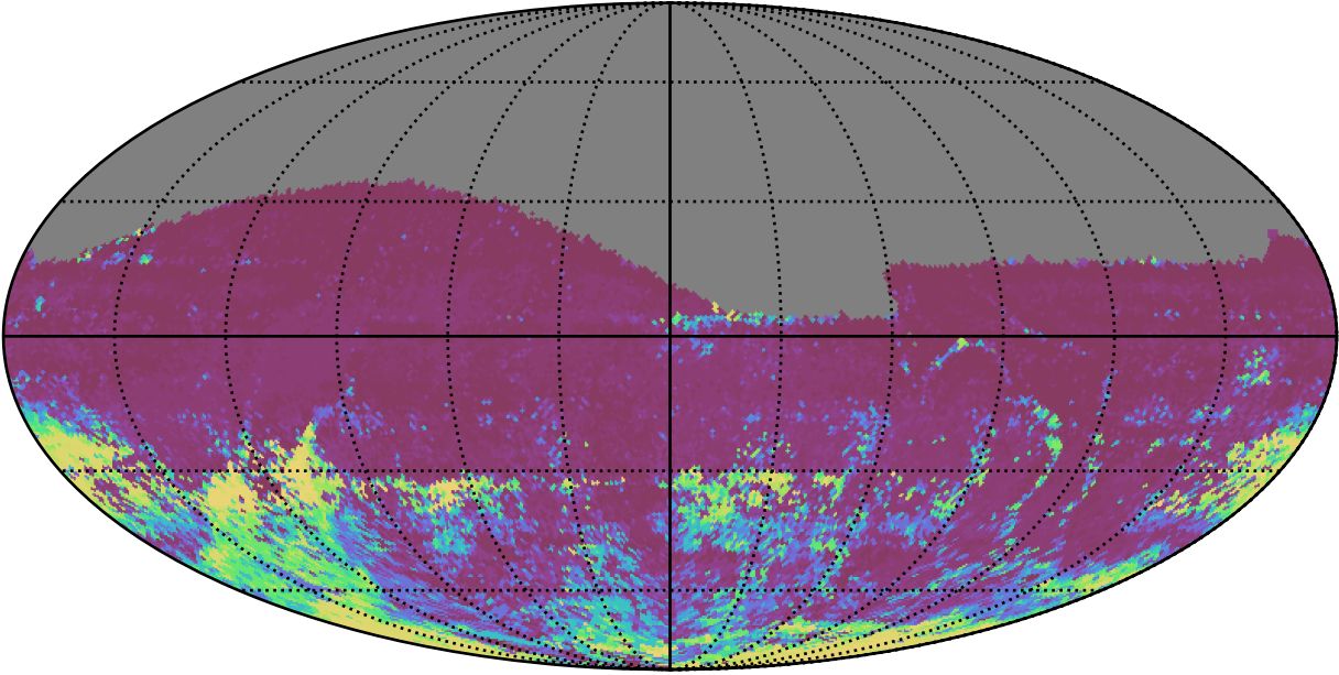
ddf_acor_sf10_lsf20_lsr50_v3.4_10yrs All sky r band: 75th Percentile Intranight Timespan
