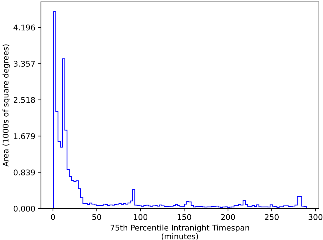
ddf_acor_sf10_lsf20_lsr50_v3.4_10yrs All sky r band: 75th Percentile Intranight Timespan
