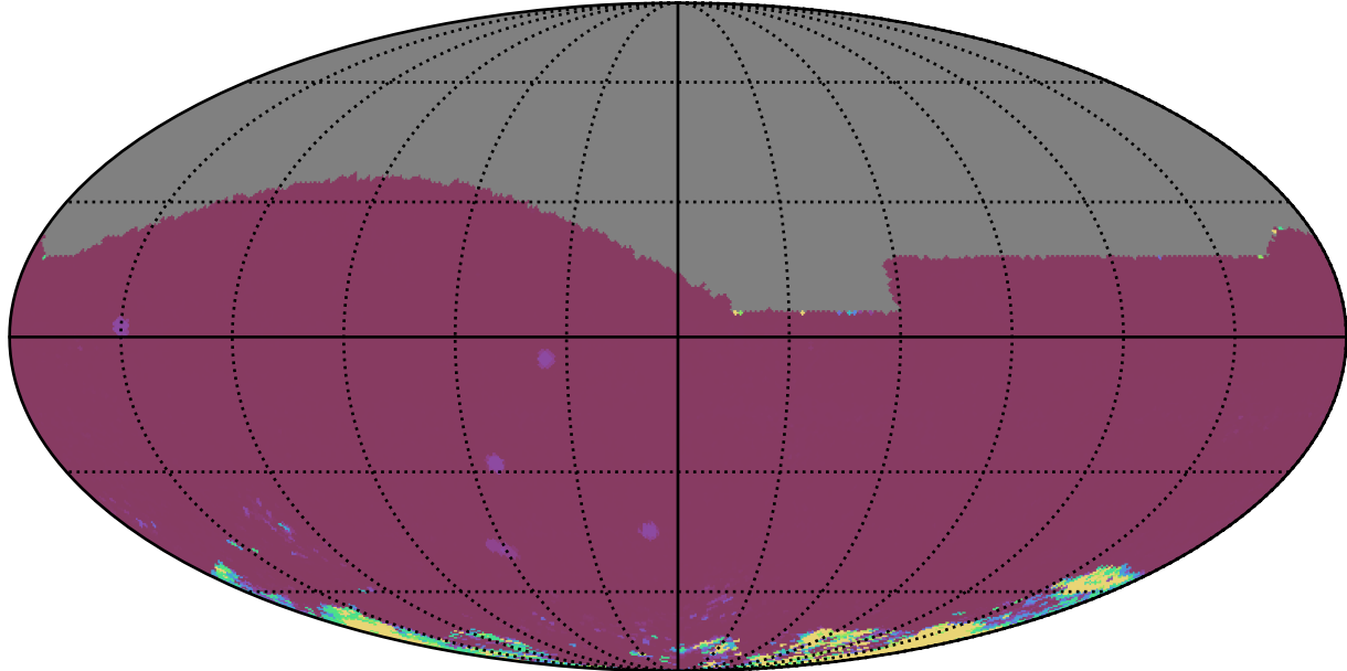
ddf_acor_sf10_lsf20_lsr50_v3.4_10yrs All sky iz bands: 75th Percentile Intranight Timespan
