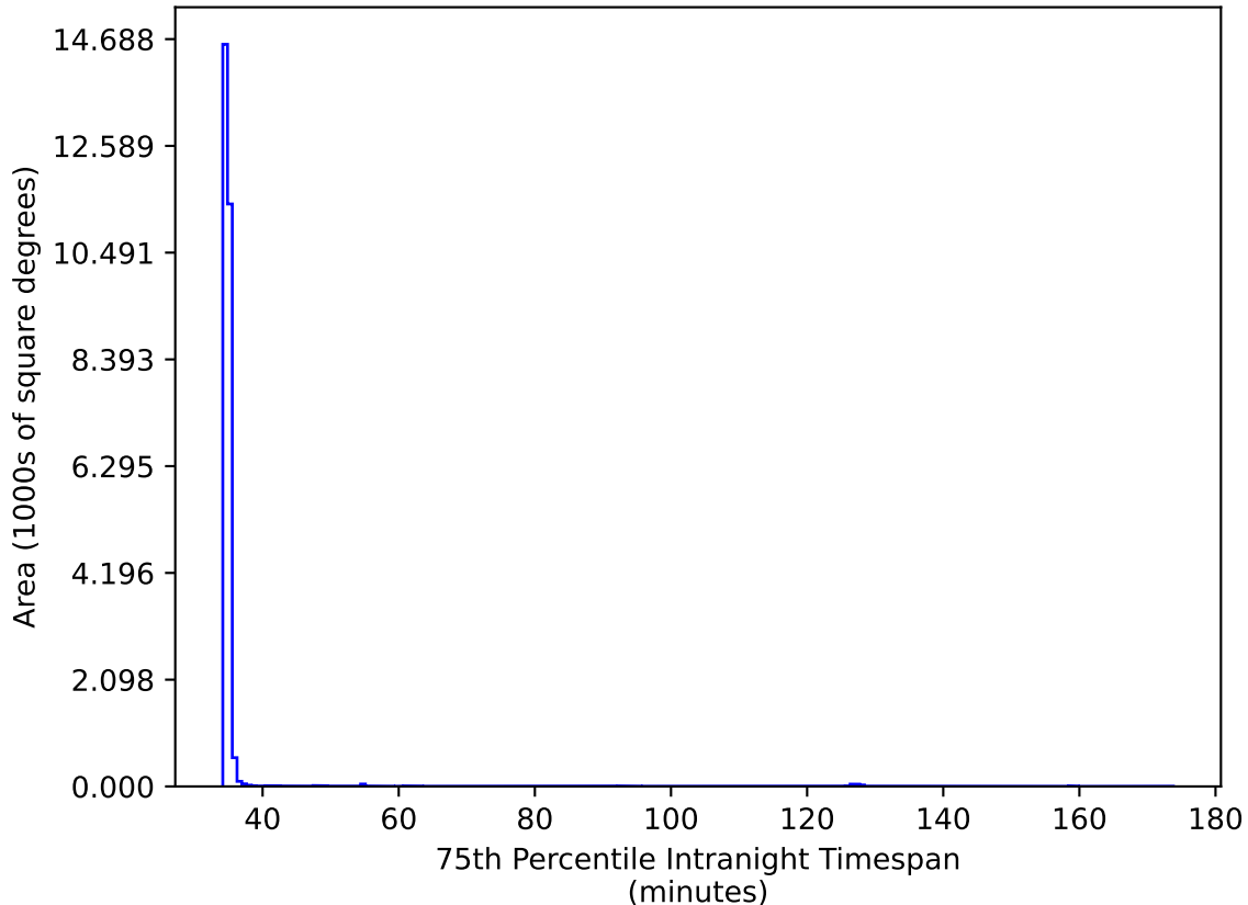
ddf_acor_sf10_lsf20_lsr50_v3.4_10yrs All sky iz bands: 75th Percentile Intranight Timespan
