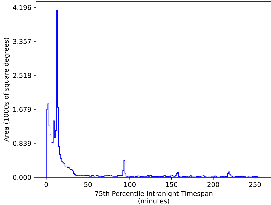
ddf_acor_sf10_lsf20_lsr50_v3.4_10yrs All sky i band: 75th Percentile Intranight Timespan
