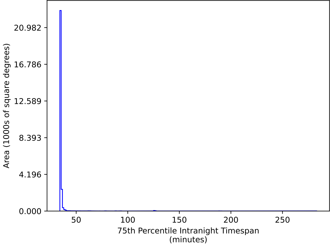
ddf_acor_sf10_lsf20_lsr50_v3.4_10yrs All sky gr bands: 75th Percentile Intranight Timespan
