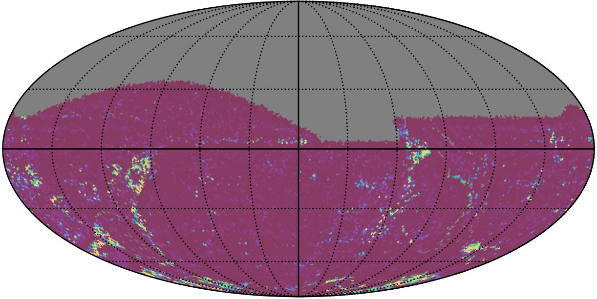
ddf_acor_sf10_lsf20_lsr50_v3.4_10yrs All sky g band: 75th Percentile Intranight Timespan
