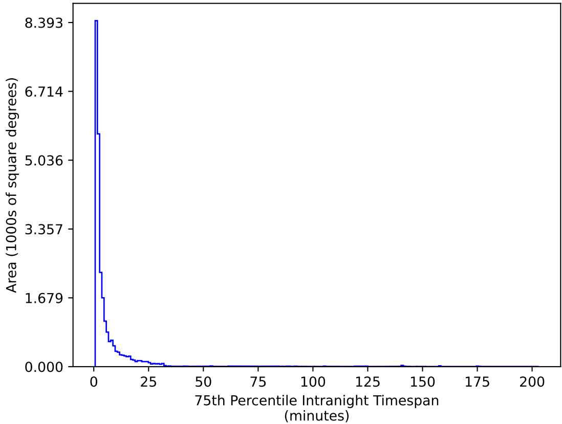
ddf_acor_sf10_lsf20_lsr50_v3.4_10yrs All sky g band: 75th Percentile Intranight Timespan
