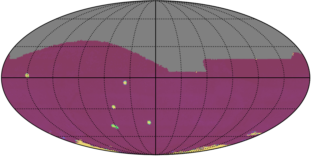
ddf_acor_sf10_lsf20_lsr50_v3.4_10yrs All sky all bands: 75th Percentile Intranight Timespan
