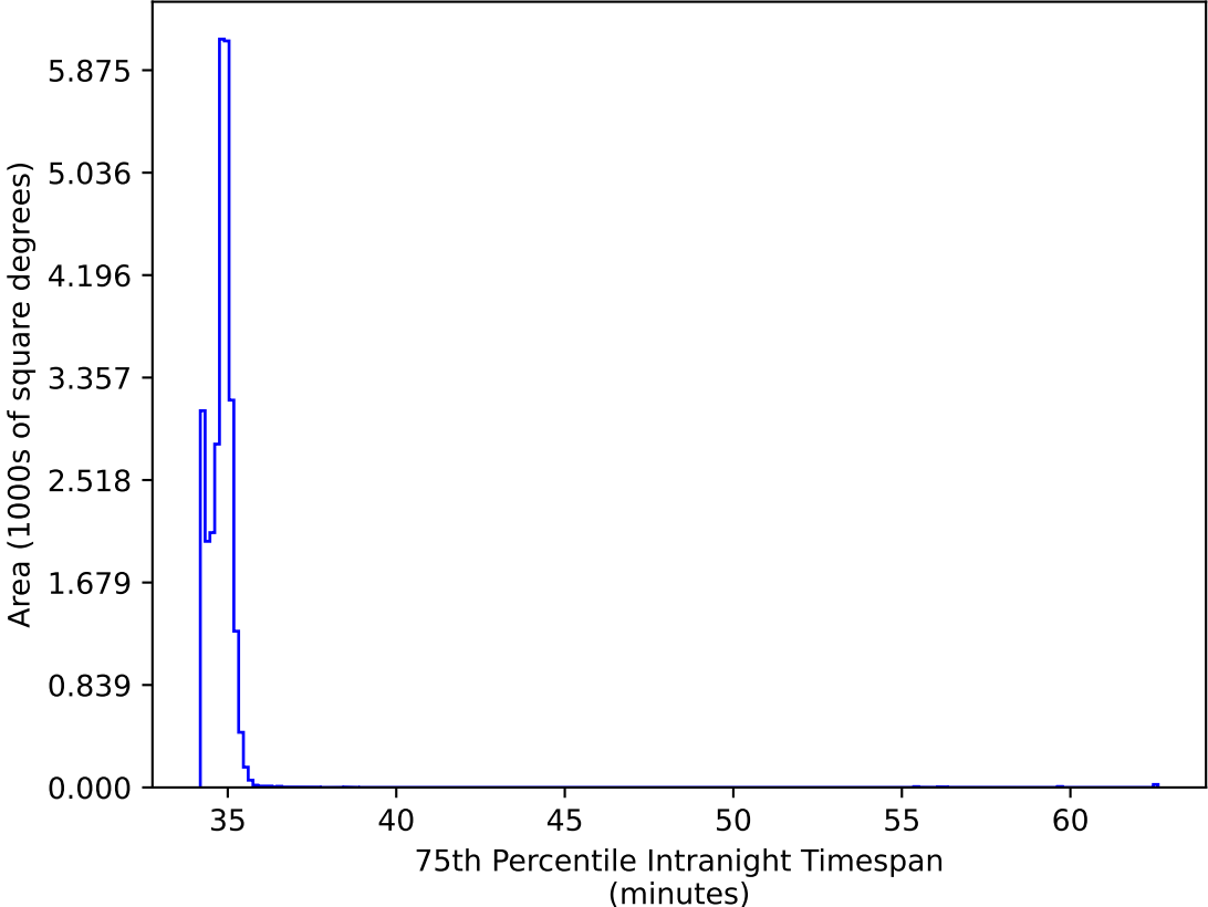
ddf_acor_sf10_lsf20_lsr50_v3.4_10yrs All sky: 75th Percentile Intranight Timespan
