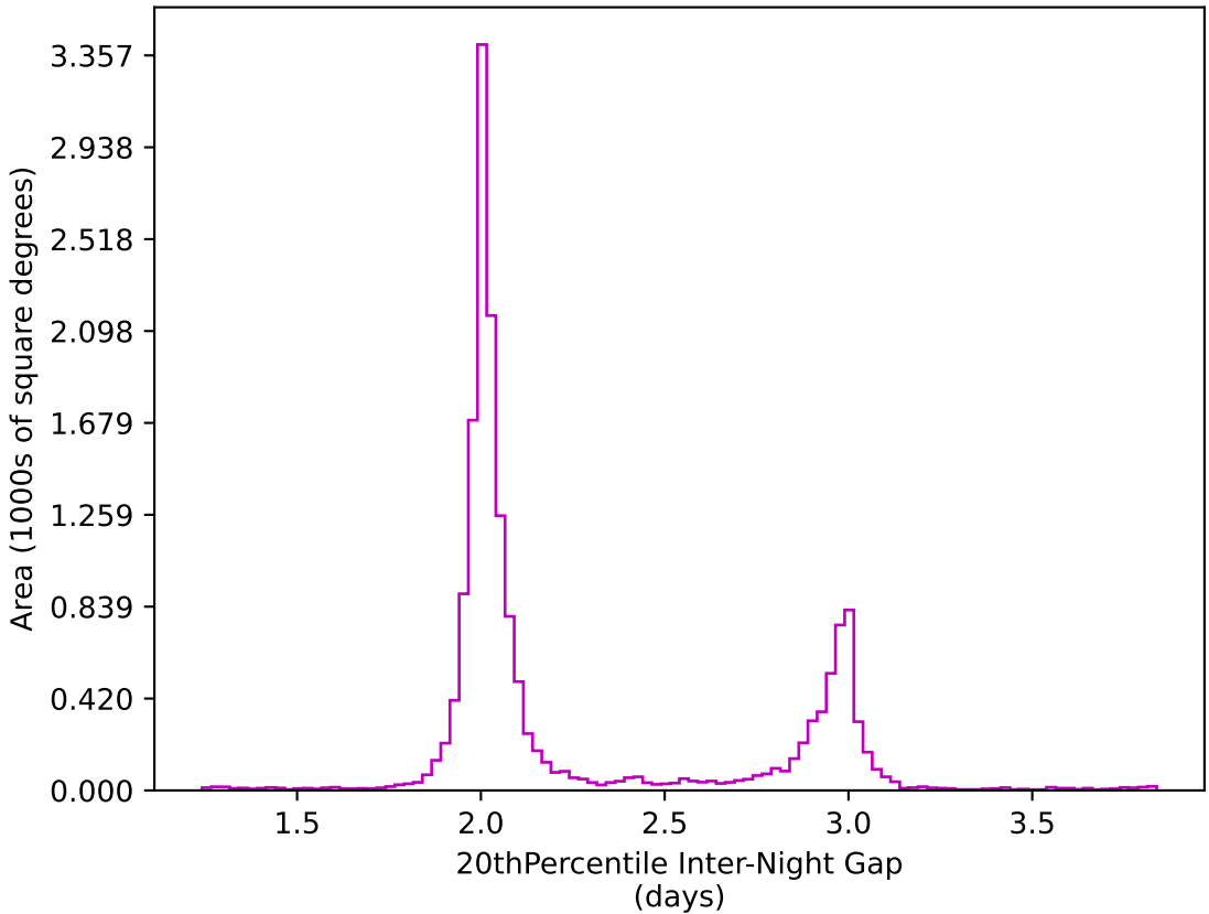
ddf_acor_sf10_lsf20_lsr50_v3.4_10yrs WFD z band: 20thPercentile Inter-Night Gap
