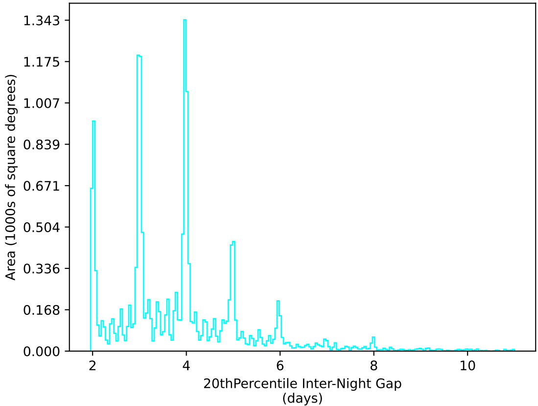
ddf_acor_sf10_lsf20_lsr50_v3.4_10yrs WFD u band: 20thPercentile Inter-Night Gap
