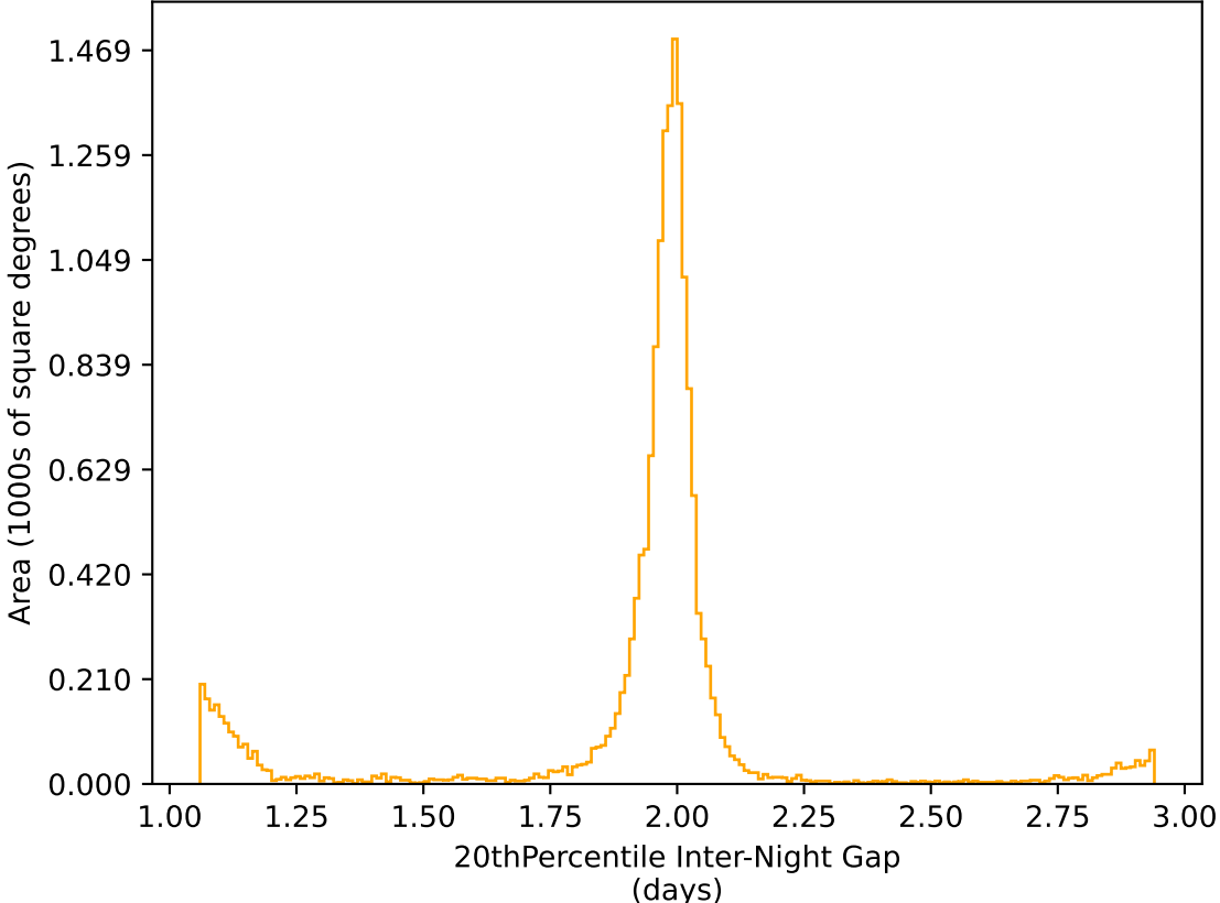
ddf_acor_sf10_lsf20_lsr50_v3.4_10yrs WFD r band: 20thPercentile Inter-Night Gap
