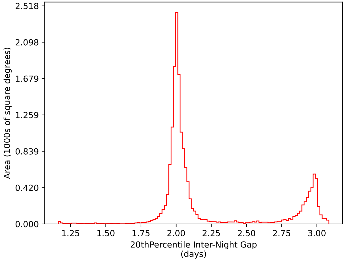
ddf_acor_sf10_lsf20_lsr50_v3.4_10yrs WFD i band: 20thPercentile Inter-Night Gap
