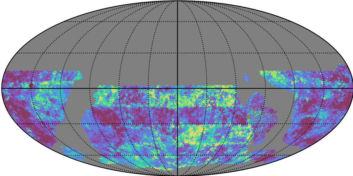
ddf_acor_sf10_lsf20_lsr50_v3.4_10yrs WFD g band: 20thPercentile Inter-Night Gap
