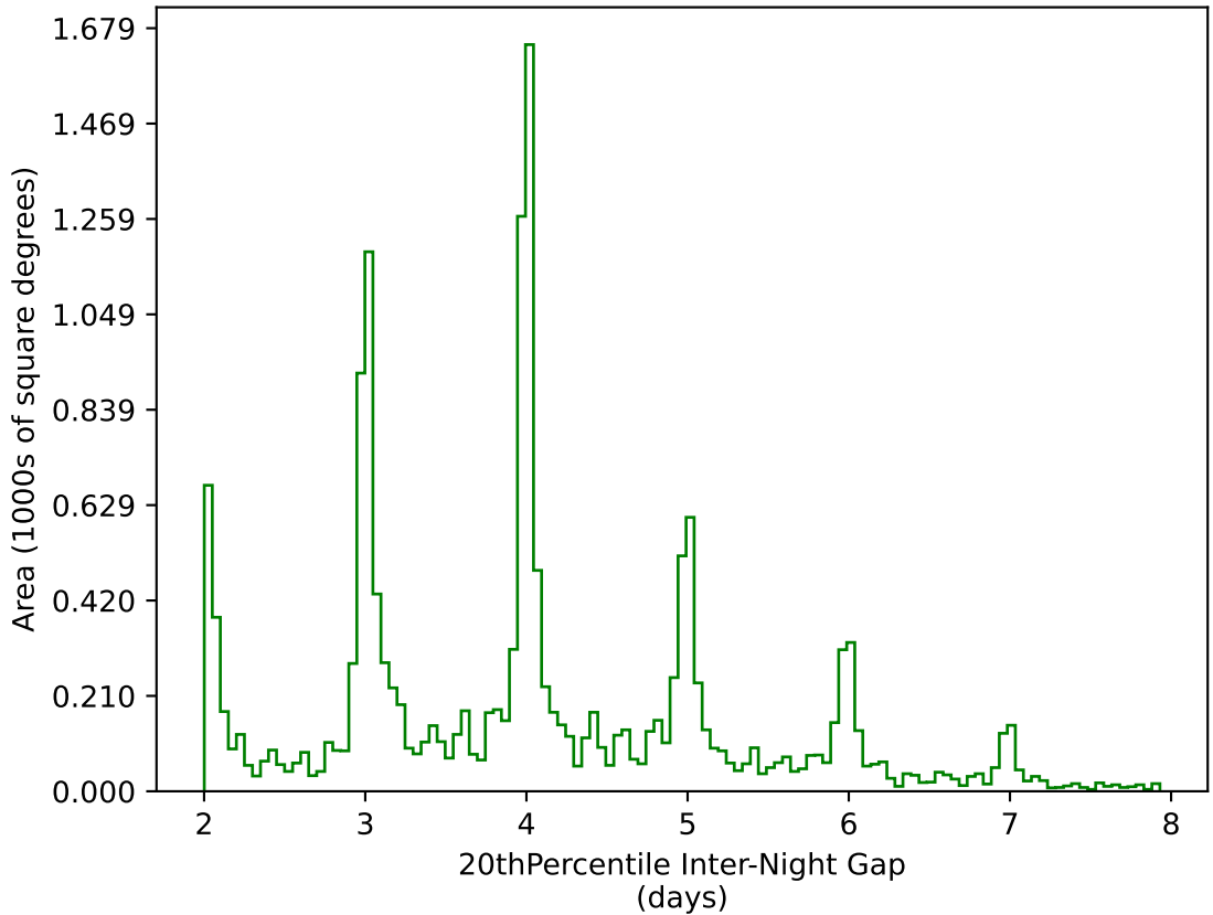
ddf_acor_sf10_ls20_lsr50_v3.4_10yrs WFD g band: 20thPercentile Inter-Night Gap
