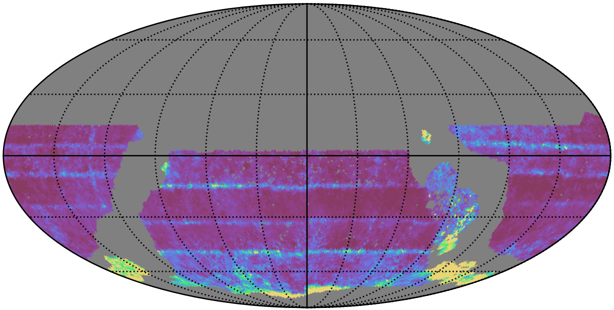
ddf_acor_sf10_lsf20_lsr50_v3.4_10yrs WFD all bands: 20thPercentile Inter-Night Gap
