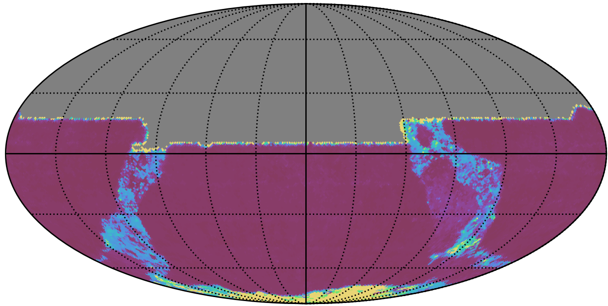
ddf_acor_sf10_lsf20_lsr50_v3.4_10yrs All sky y band: 20thPercentile Inter-Night Gap
