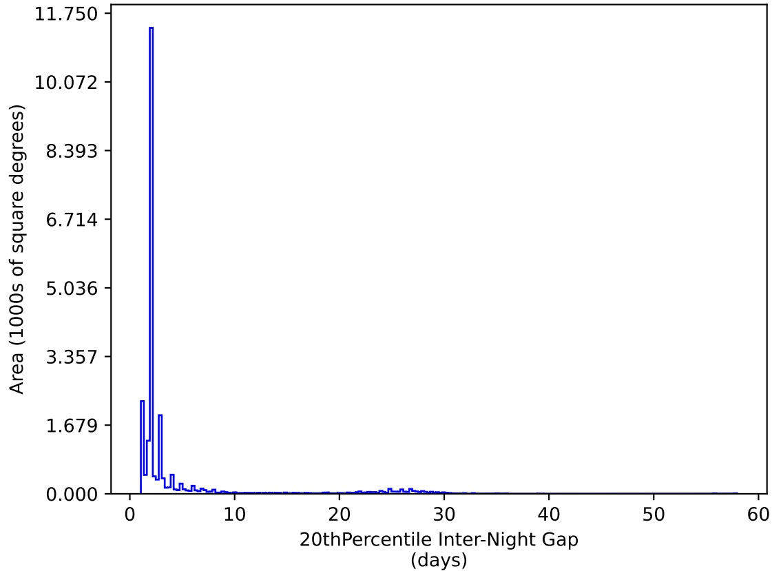
ddf_acor_sf10_lsf20_lsr50_v3.4_10yrs All sky y band: 20thPercentile Inter-Night Gap
