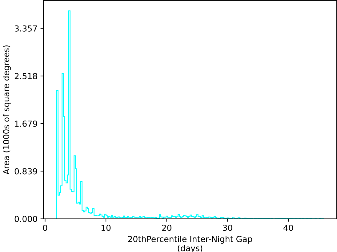
ddf_acor_sf10_lsf20_lsr50_v3.4_10yrs All sky u band: 20thPercentile Inter-Night Gap
