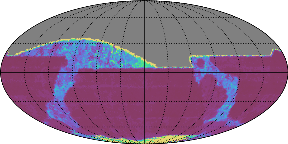
ddf_acor_sf10_lsf20_lsr50_v3.4_10yrs All sky i band: 20thPercentile Inter-Night Gap
