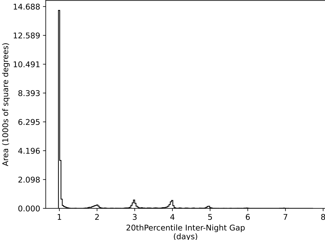
ddf_acor_sf10_lsf20_lsr50_v3.4_10yrs All sky all bands: 20thPercentile Inter-Night Gap
