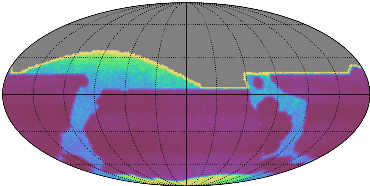
ddf_acor_sf10_lsf20_lsr50_v3.4_10yrs : properMotion
