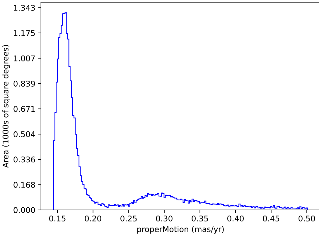
ddf_acor_sf10_ls20_lsr50_v3.4_10yrs : properMotion
