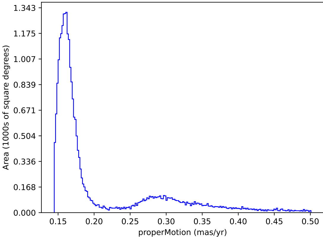
ddf_acor_sf10_ls20_lsr50_v3.4_10yrs : properMotion
