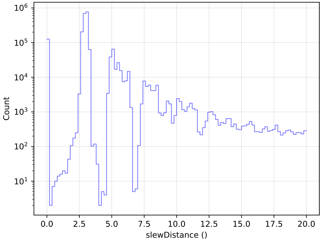
ddf_acor_sf10_lsf20_lsr50_v3.4_10yrs All visits: Zoom Slew Distance Histogram
