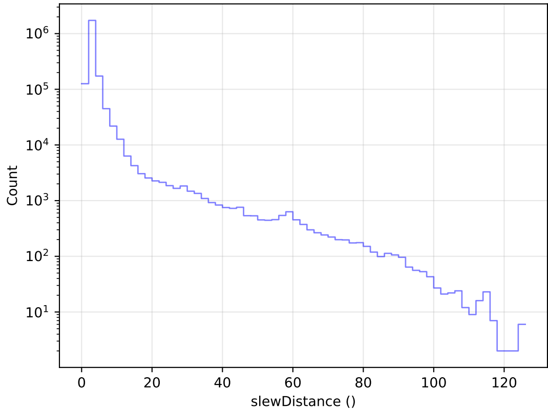
ddf_acor_sf10_lsf20_lsr50_v3.4_10yrs All visits: Slew Distance Histogram
