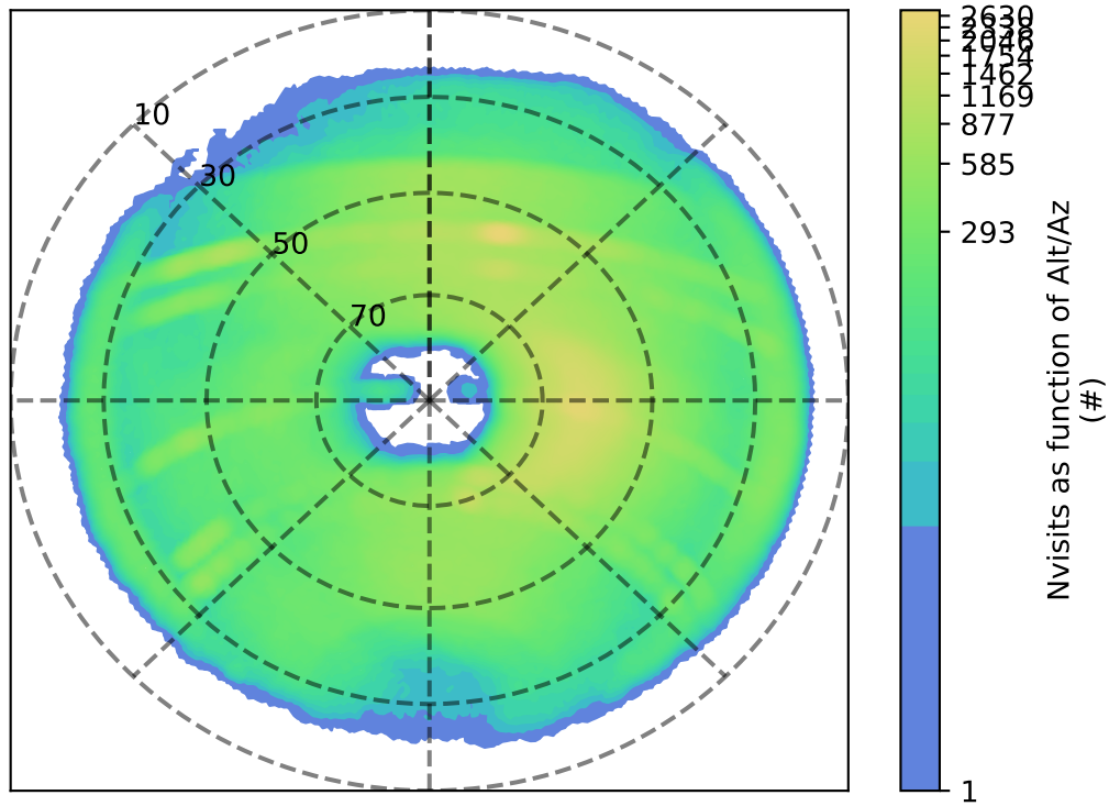
ddf_acor_sf10_lsf20_lsr50_v3.4_10yrs z: Nvisits as function of Alt/Az
