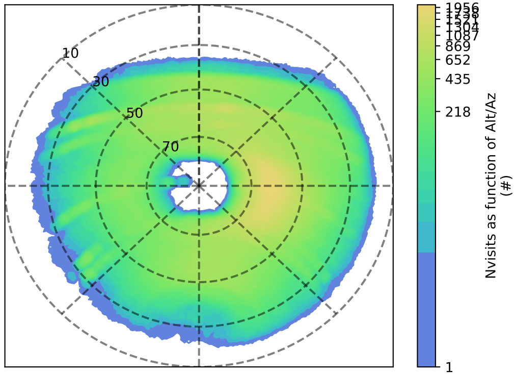
ddf_acor_sf10_lsf20_lsr50_v3.4_10yrs y: Nvisits as function of Alt/Az
