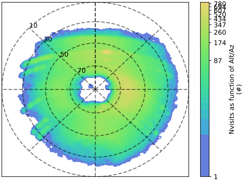
ddf_acor_sf10_lsf20_lsr50_v3.4_10yrs u: Nvisits as function of Alt/Az
