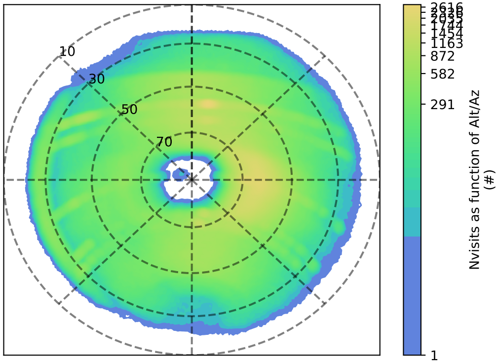
ddf_acor_sf10_ls20_lsr50_v3.4_10yrs r: Nvisits as function of Alt/Az
