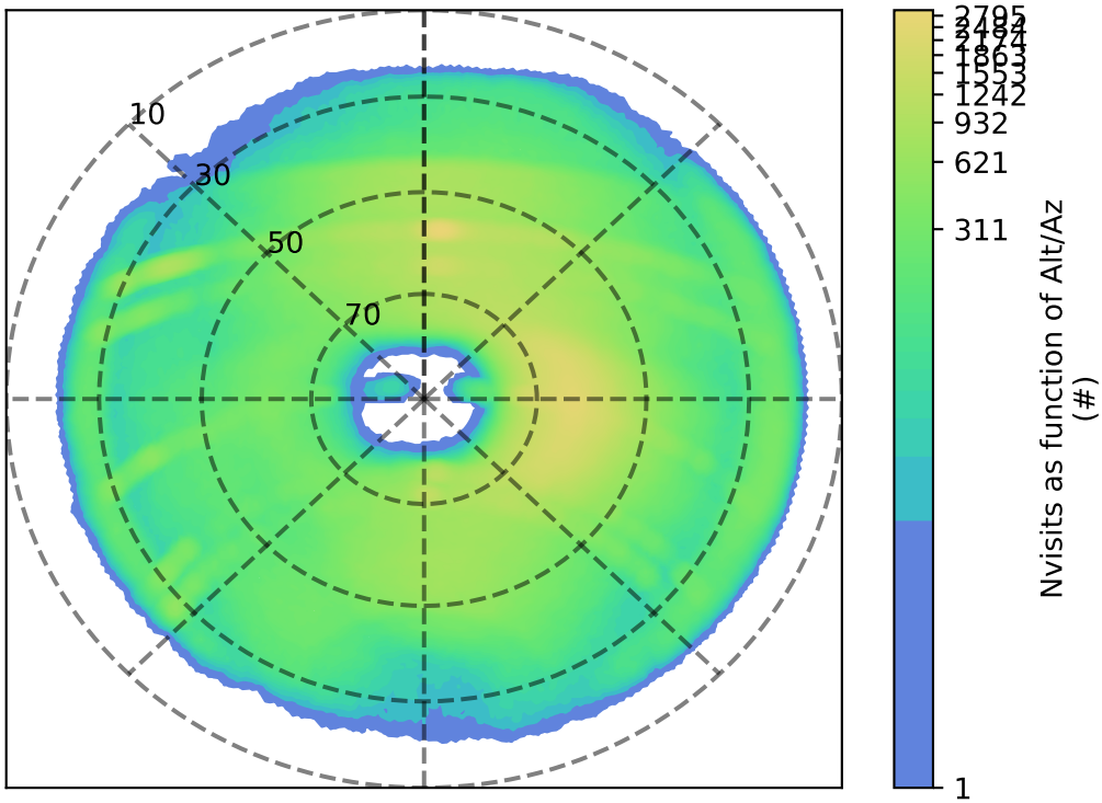
ddf_acor_sf10_ls20_lsr50_v3.4_10yrs i: Nvisits as function of Alt/Az
