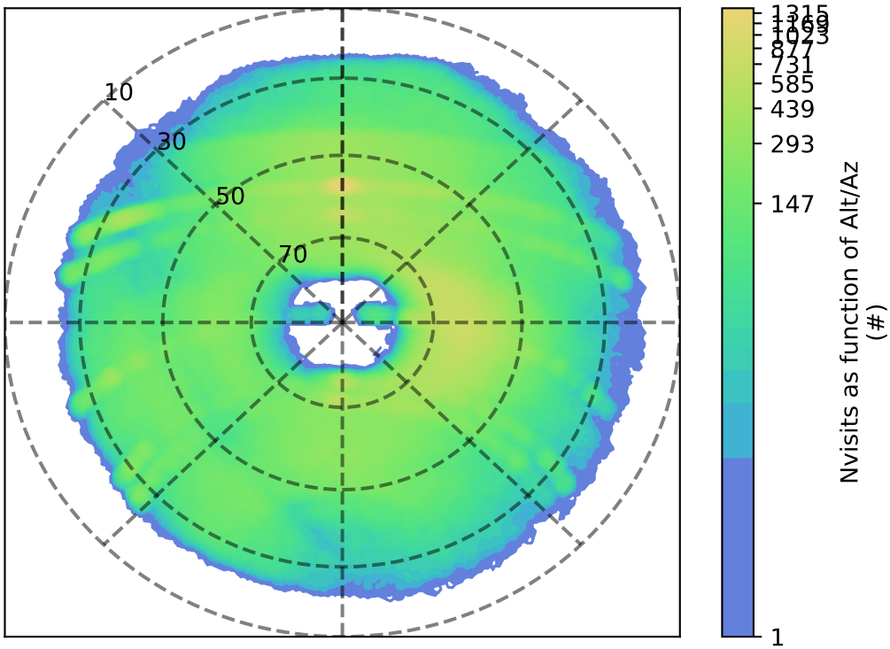
ddf_acor_sf10_lsf20_lsr50_v3.4_10yrs g: Nvisits as function of Alt/Az
