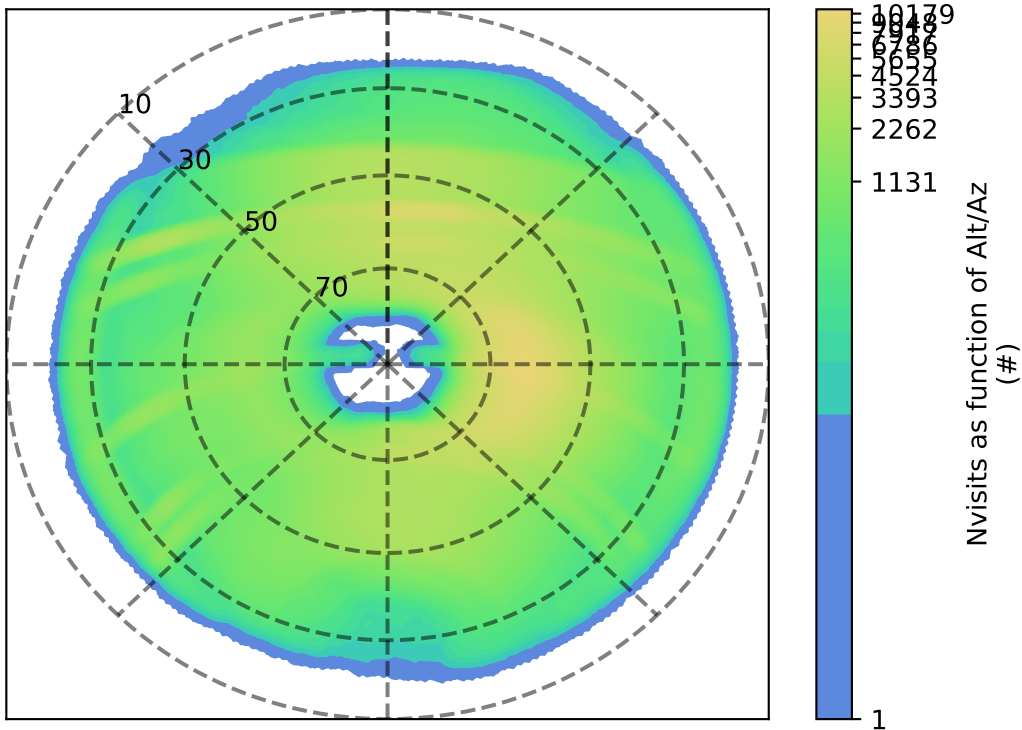
ddf_acor_sf10_lsf20_lsr50_v3.4_10yrs : Nvisits as function of Alt/Az
