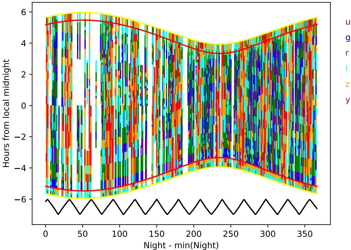
ddf_acor_sf10_lsf20_lsr50_v3.4_10yrs year 9-10: Hourglass
