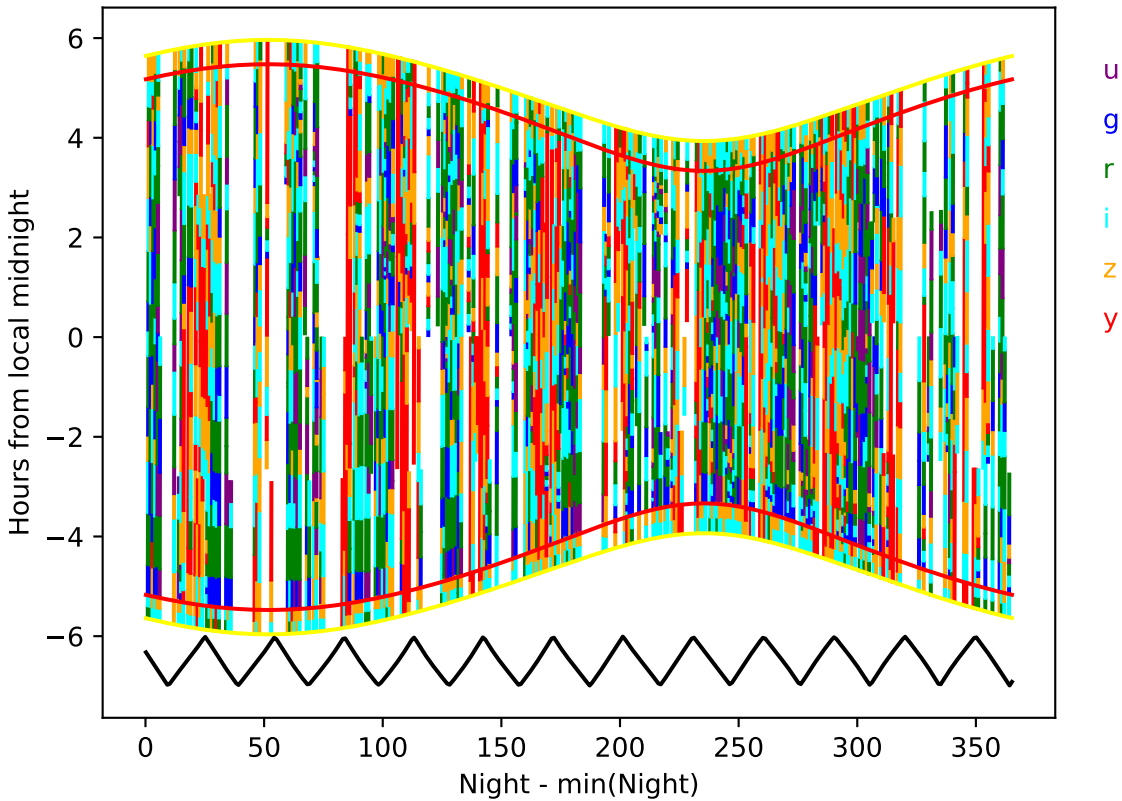
ddf_acor_sf10_lsf20_lsr50_v3.4_10yrs year 7-8: Hourglass
