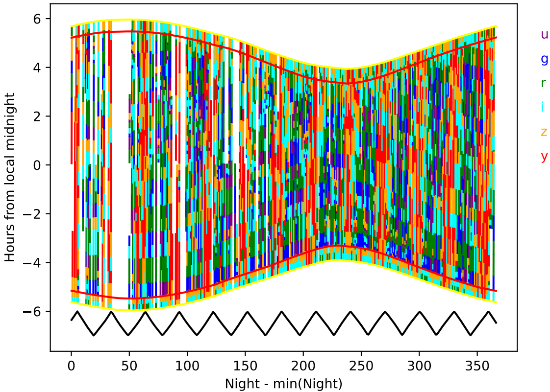
ddf_acor_sf10_lsf20_lsr50_v3.4_10yrs year 6-7: Hourglass
