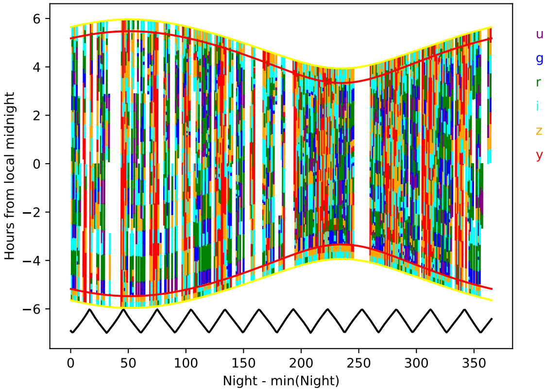
ddf_acor_sf10_lsf20_lsr50_v3.4_10yrs year 5-6: Hourglass
