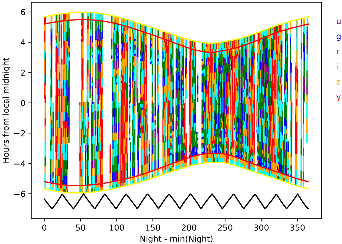
ddf_acor_sf10_lsf20_lsr50_v3.4_10yrs year 4-5: Hourglass
