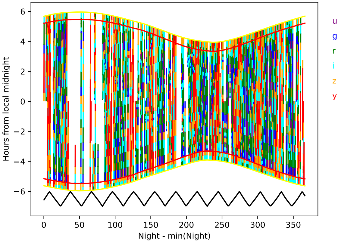
ddf_acor_sf10_lsf20_lsr50_v3.4_10yrs year 3-4: Hourglass
