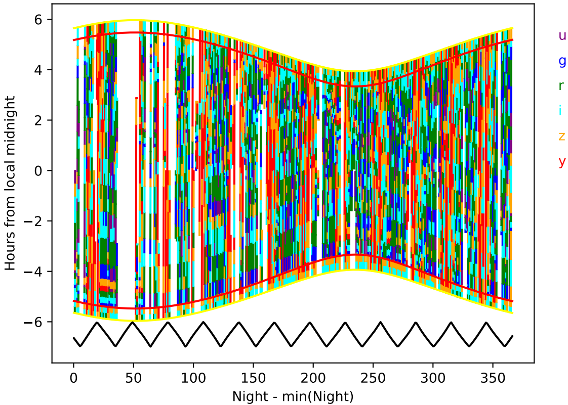
ddf_acor_sf10_lsf20_lsr50_v3.4_10yrs year 2-3: Hourglass
