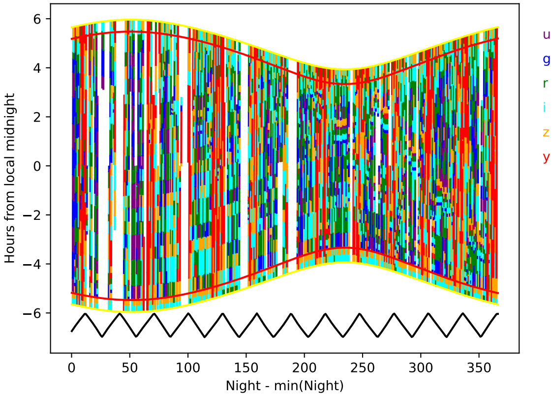
ddf_acor_sf10_lsf20_lsr50_v3.4_10yrs year 0-1: Hourglass
